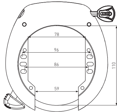
4750S / 4750SL
