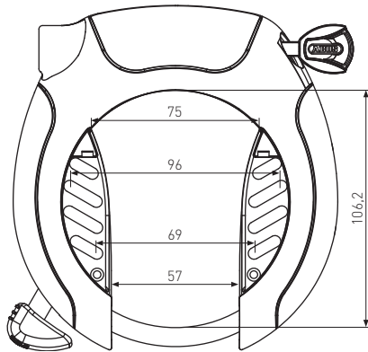
4750X / 4750XL
